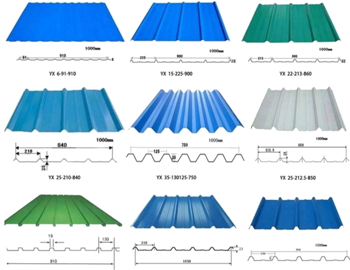
Trapezoidal roofing sheet
